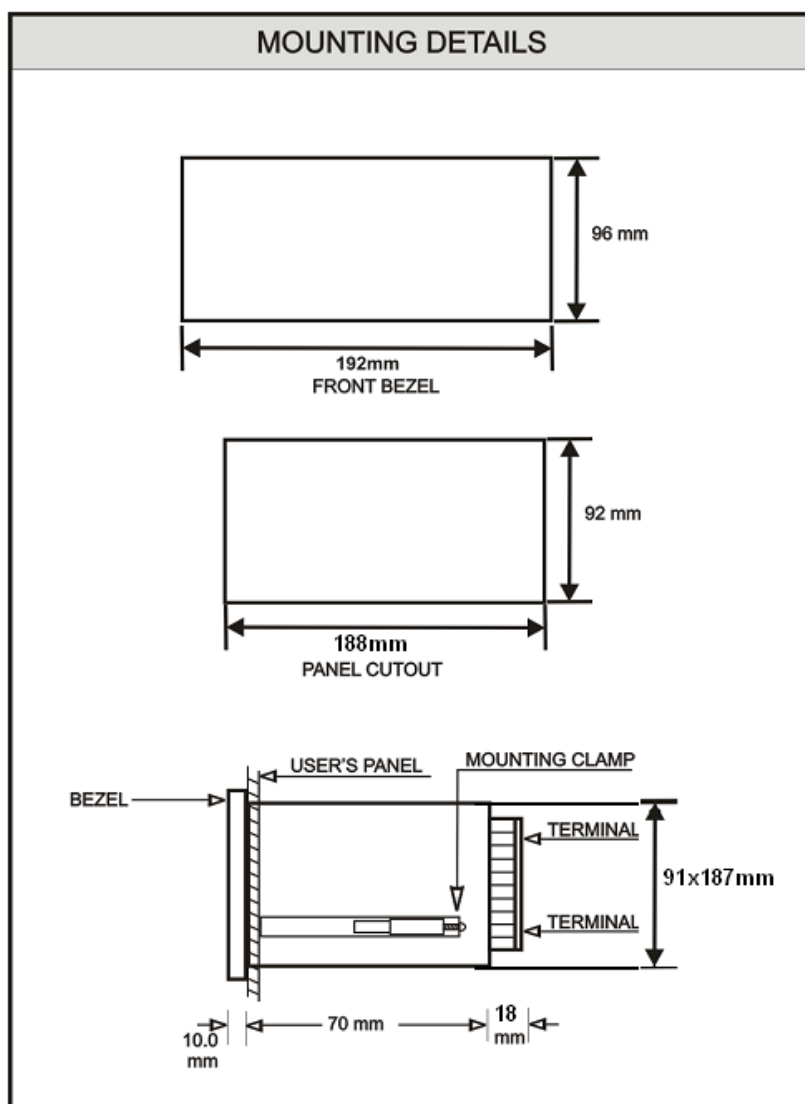
Fig 3.2: Mounting Details
